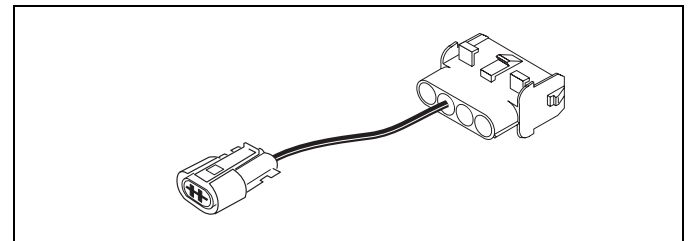
Fig. 2: Test adapter for Thermo 90 S/ST, Thermo Top Evo and Thermo 50 MAN/trade heaters, order no. 92556B
