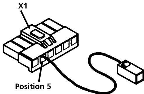
New Adapter (Pigtail) P/N 5000007A
